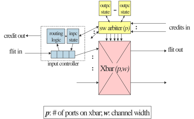
Figure 2. Canonical wormhole router architecture.
