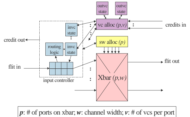
Figure 3. Canonical virtual-channel router architecture.
