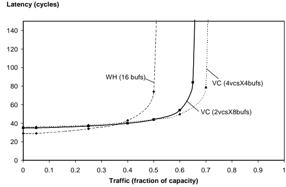
Figure 8. Latency-throughput curves of wormhole and virtual-channel routers with 16 buffers per input port. The routers are pipelined as prescribed by the proposed pipelined router model.
